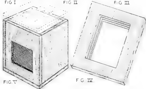
An easily made box for exposing developing papers; also for a dark-room lantern
